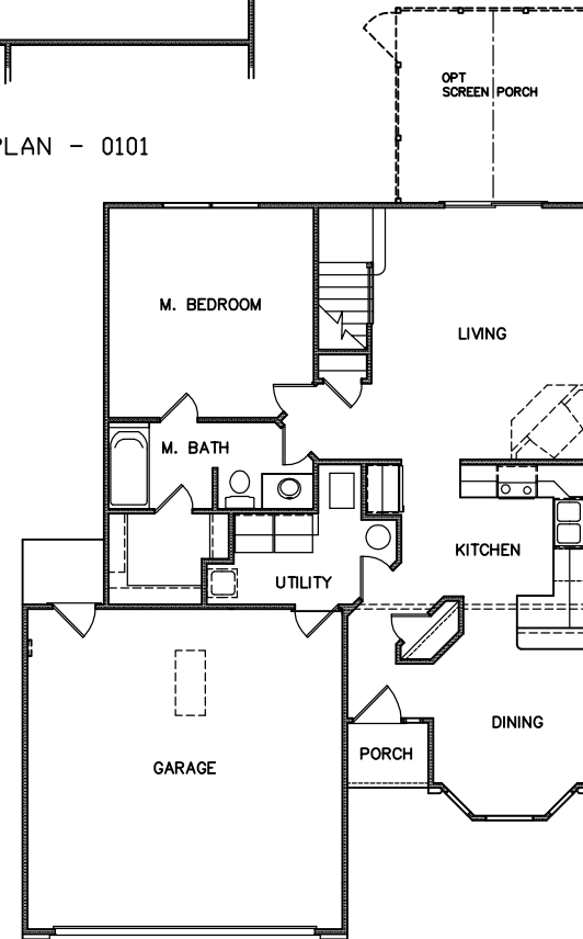
FIRST FLOOR PLAN - 0101 910 SF 35' W x 45' D
