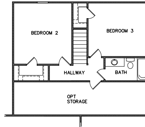
SECOND FLOOR PLAN - 0101 506 SF
