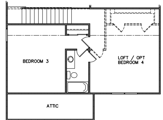
SECOND FLOOR PLAN - 0104 633 SF
