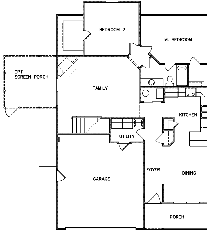
FIRST FLOOR PLAN - 0104 1251 SF 35' W x 52' D
