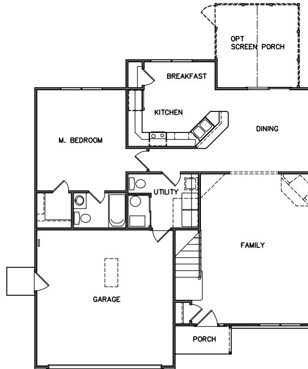
FIRST FLOOR PLAN - 0110 1143 SF 40' W x 44' D
