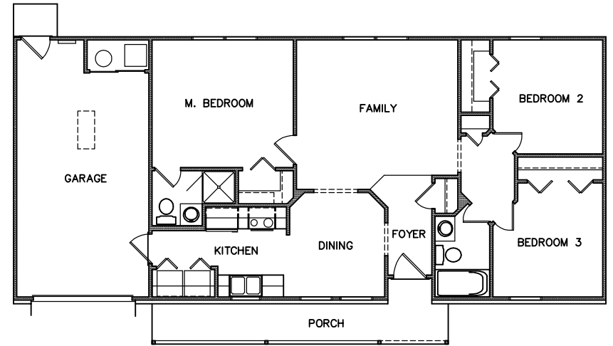
FLOOR PLAN - 0112 992 SF 54' W x 28' D
