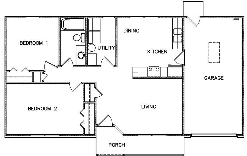
FLOOR PLAN - 0113 855 SF 48' W x 28' D
