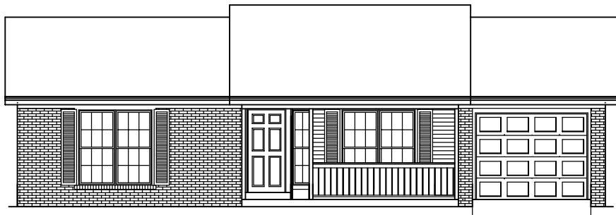
FRONT ELEVATION - C - 0113
