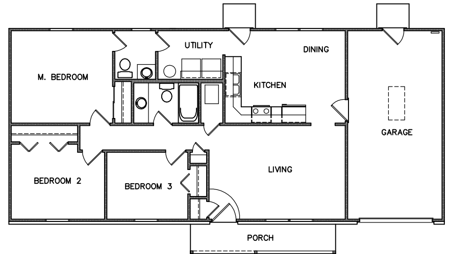
FLOOR PLAN - 0114 1008 SF 54' W x 28' D
