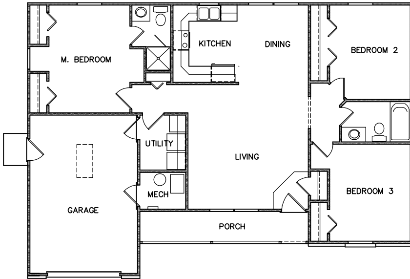
FLOOR PLAN - 0115 1135 SF 48' W x 34' D
