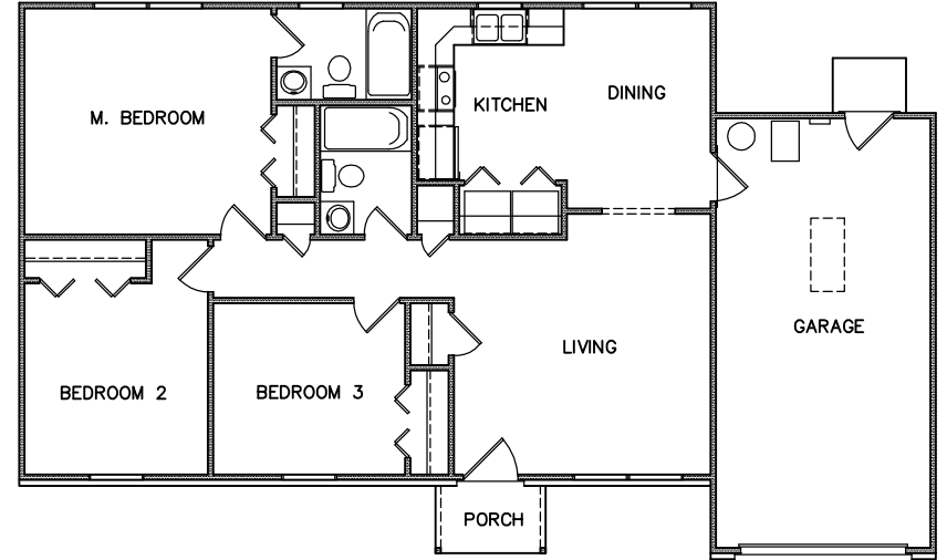
FLOOR PLAN - 0116 988 SF 50' W x 30' D
