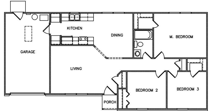
FLOOR PLAN - 0117 1020 SF 54' W x 26' D
