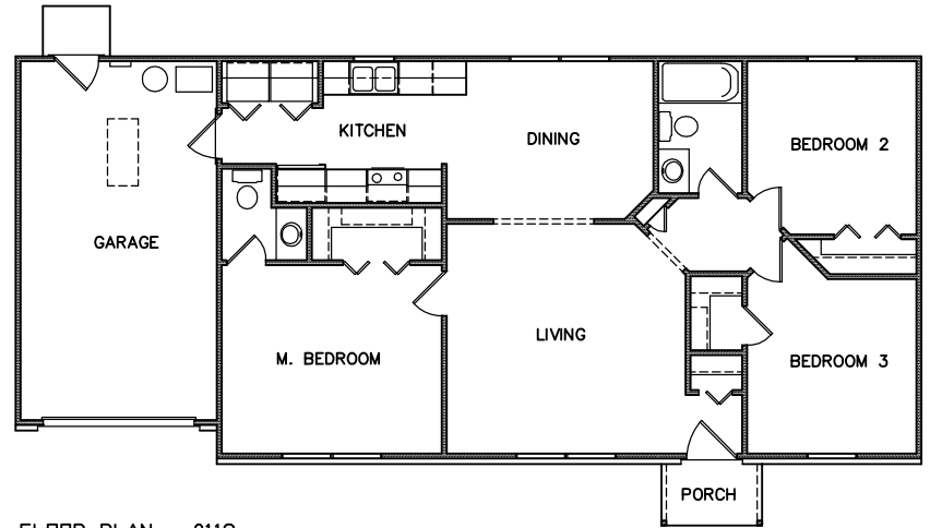
FLOOR PLAN - 0118 1008 SF 54' W x 28' D
