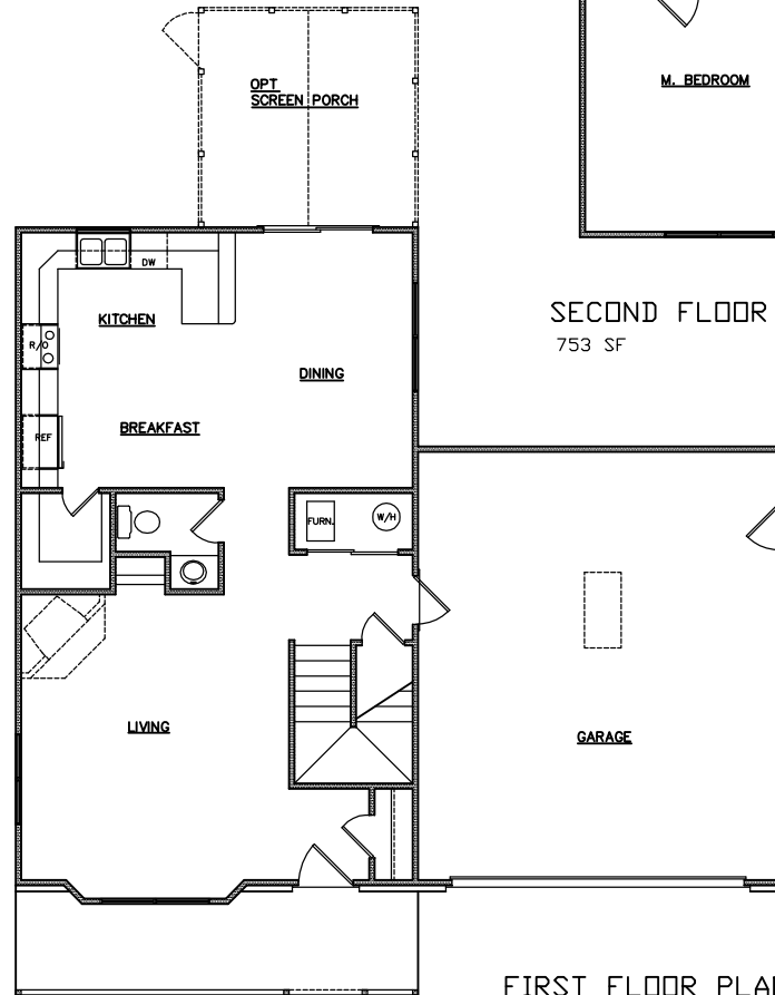
FIRST FLOOR PLAN - 0201 801 SF 42' W x 42' D
