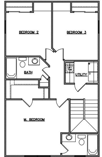
SECOND FLOOR PLAN - 0201 753 SF
