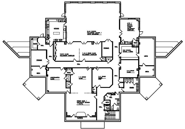
STARTER CHURCH PLAN 07 9,049 SF UP 264 SEATS 8,515 SF DN
