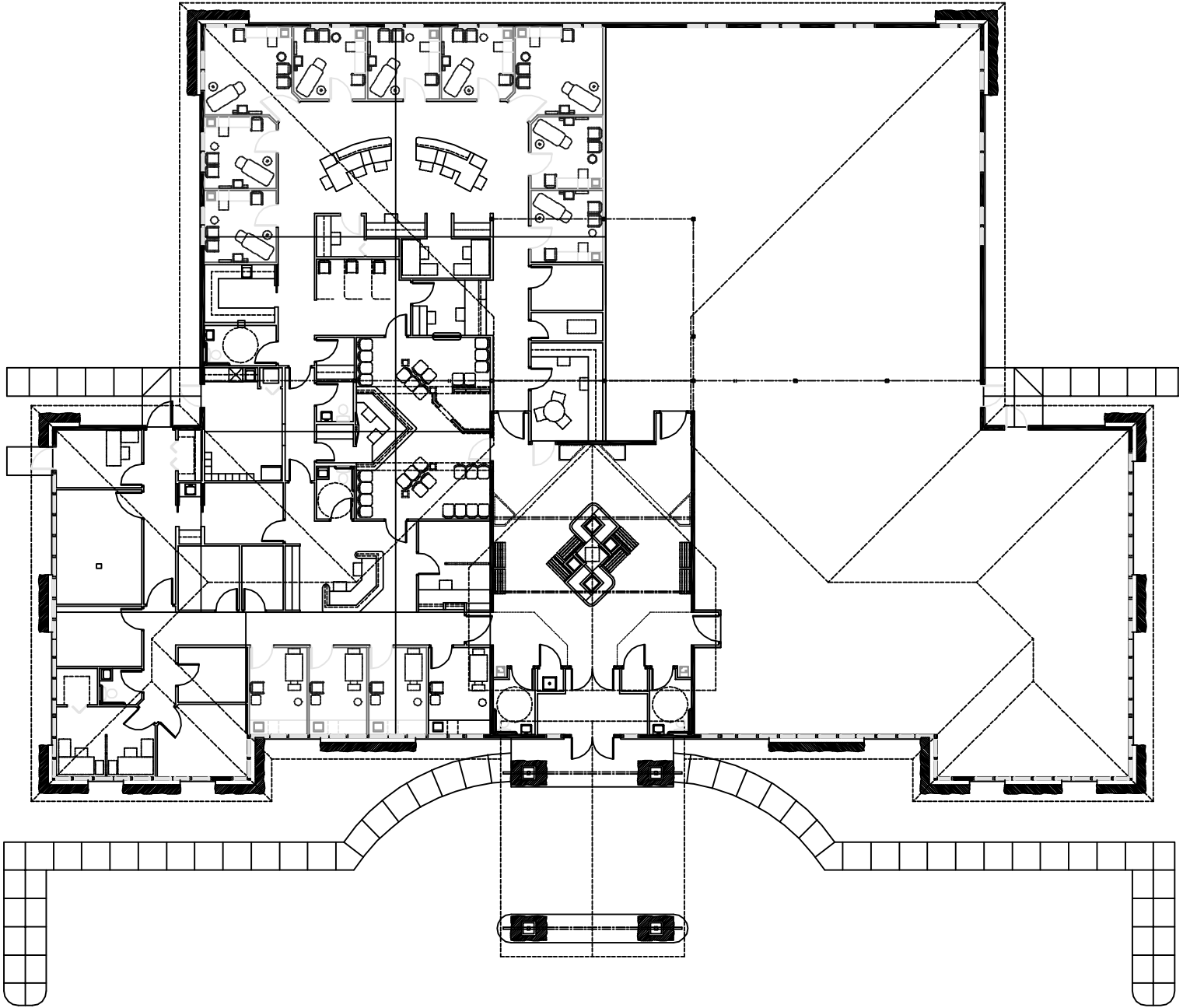
STARTER CLINIC PLAN 02 13,373 SF
